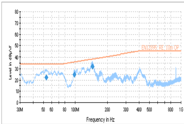
Figure 14: test result(Vertical)
